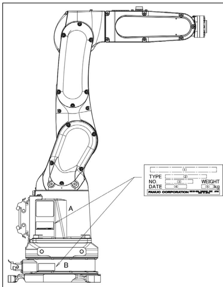
Position of label indicating mechanical unit and force sensor specification number
